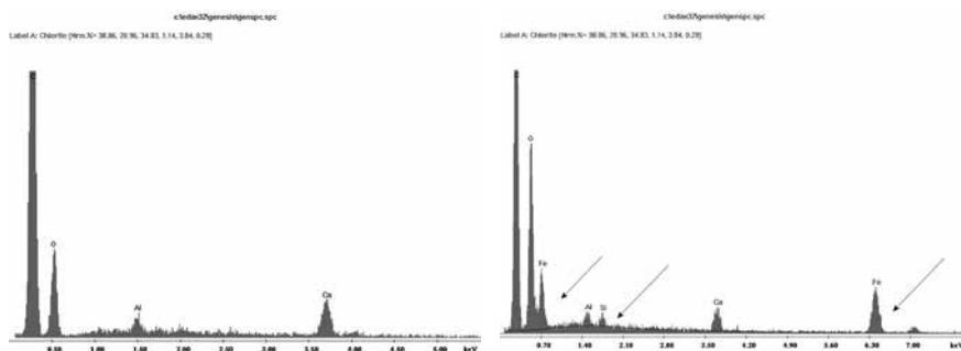
Figure 13. Spectrograms of the elemental composition of the paste stroke of the ballpoint pen (a) and the particles of the electrophotographic powder on the test stroke (b). The arrows indicate the peaks of two- and trivalent iron, and silicon
